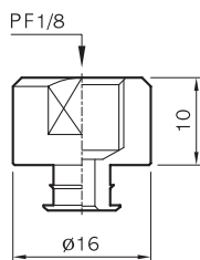
18F-1
